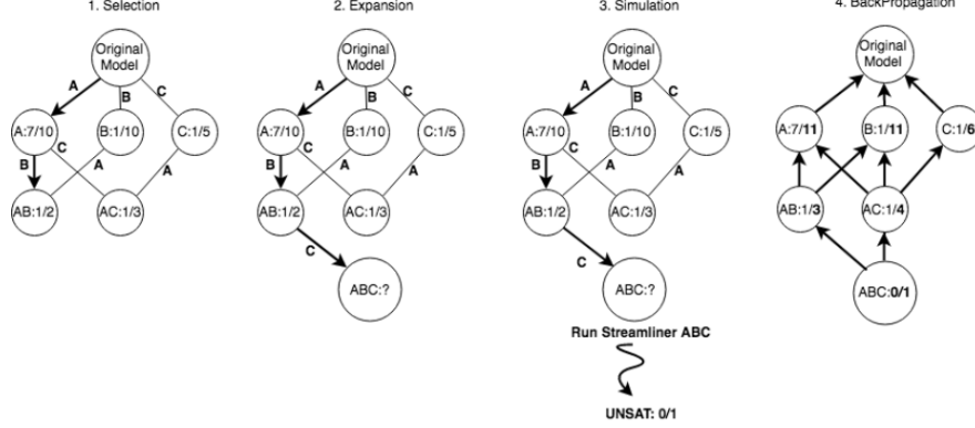
Figure 10: MOMCTS-DOM operating on the streamliner lattice. A, B and C refer to single candidate streamliners generated from the original ESSENCE specification. As MOMCTS-DOM descends down through the lattice the streamliners are combined through the conjunction of the individual streamliners (AB, ABC). The nodes are labelled with CDD reward value divided by the number of times visited.
