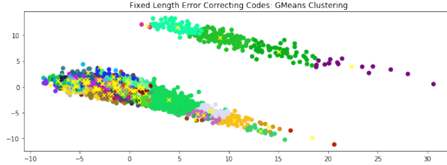
Figure 8: GMeans clustering results on the instance feature space (projected to 2-dimensional space by PCA) for the Fixed Length Error Correcting Codes problem with CHUFFED. Each color represents a cluster.
