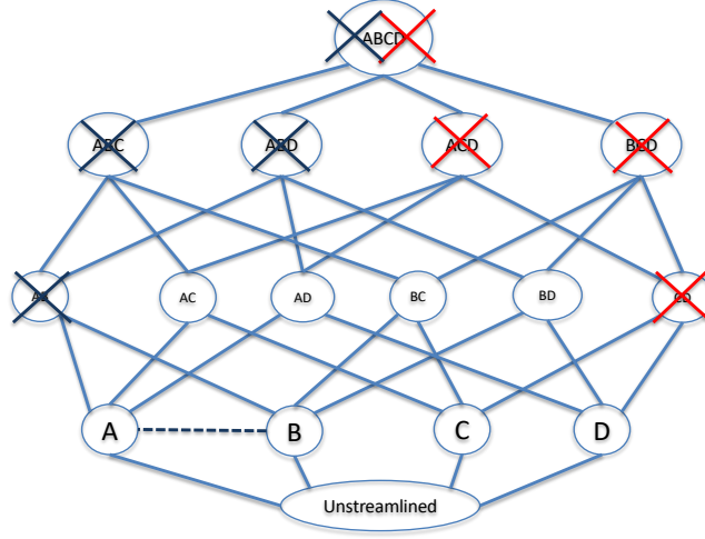
Figure 9: The power set of singleton candidate streamliners is explored to identify combinations that result in powerful streamlined specifications. Starting from an empty set of streamliners (the unstreamlined model), new streamliners are gradually added. If small sets of streamliners that fail to retain solutions are identified, such as CD , all supersets can be pruned from the search, vastly reducing the number of vertices to be explored. Streamliners A and B are tagged (Section 3) mutually exclusive, and so no streamliner combinations containing both are evaluated.
