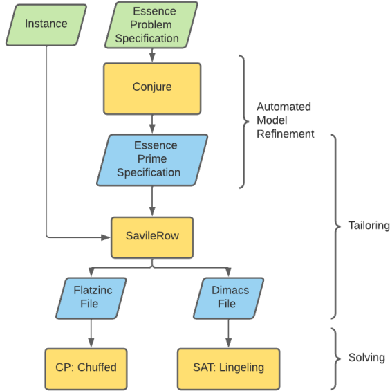
Figure 2: Solving a problem instance using a streamlined Essence specification. CONJURE is run once for a streamlined model, whereas SAVILE ROW and the selected solver is run once per instance. The streamliner that is provided as input to CONJURE is generated by a separate call to CONJURE as part of Phase 1 (Candidate Streamliner Generation).
