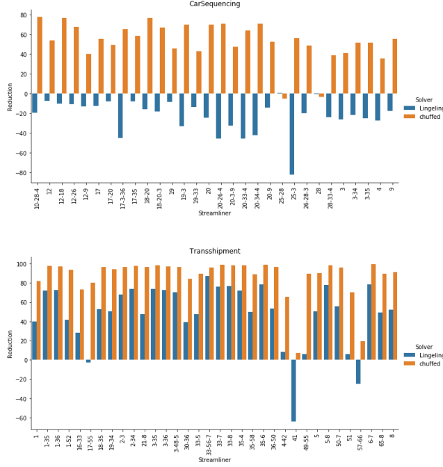
Figure 11: For Transshipment and CarSequencing the portfolios generated during the CHUFFED streamliner search are tested on LINGELING on the same set of test instances. The Average Reduction across the two portfolios are represented for both paradigms. The same set of test instances are used so that any variation in the reductions of the streamliners is purely due to the different setting.
