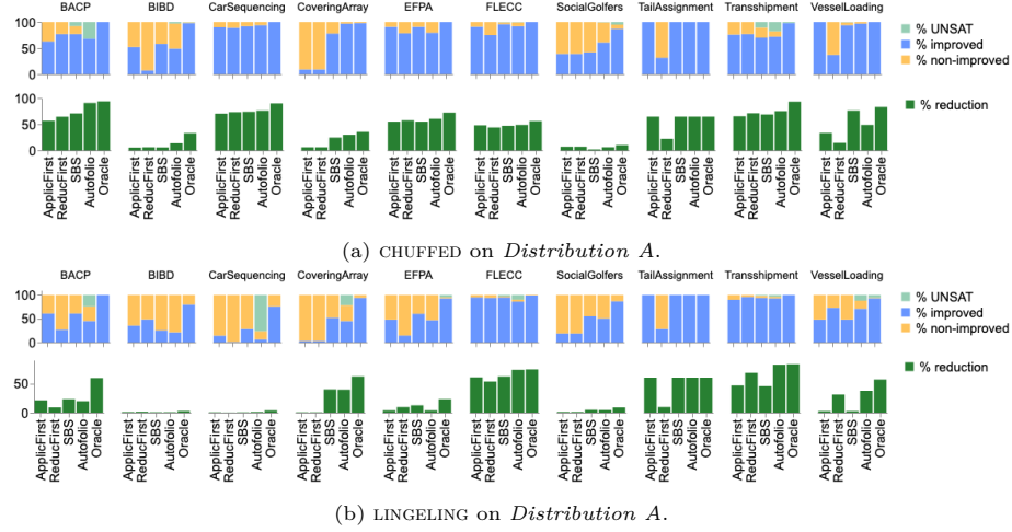
Figure 12: Results with CHUFFED and LINGELING on Distribution A . The top of each pair of charts shows how frequently the associated approach produces an improvement (% improved), and also indicates the reason for failure to improve on the remainder of the instances: the instance was rendered unsatisfiable (% UNSAT), or the search completed more slowly than the unstreamlined model (% non-improved). The bottom of each pair of charts shows the magnitude of the solving time reduction on those instances where an improvement was obtained (% reduction). Hence, care must be taken when comparing approaches, since an infrequently applicable approach may do well on the few instances it does improve (e.g. the lexicographic scheduling approaches on the Social Golfers Problem). The best approaches are both frequently applicable and result in a large search reduction.
