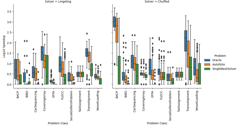
Figure 14: Distribution of speedup values (in base 10 logarithmic scale) for the Oracle, AutoFolio and SingleBestSolver on Distribution B
