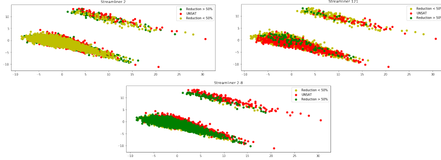
Figure 7: Performance of three example streamliners on the training set of 4647 instances generated for the Fixed Length Error Correcting Code problem with CHUFFED. Each two dimensional plot is a projection of the original multi-dimensional instance feature space via Principal Component Analysis.
