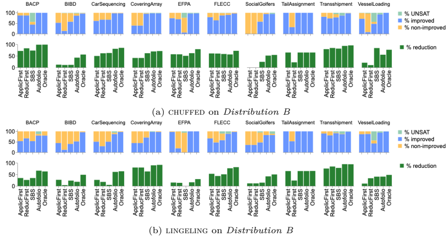
Figure 13: Results with CHUFFED and LINGELING on Distribution B . Detailed on meaning of the plots are described in Figure 12.
